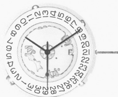
3 Hands Cal. 6003.D 2.50 mm
